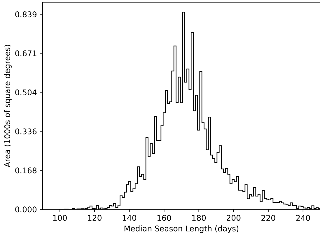
ddf_acor_sf25_lsf30_lsr10_v3.4_10yrs WFD all bands: Median Season Length
