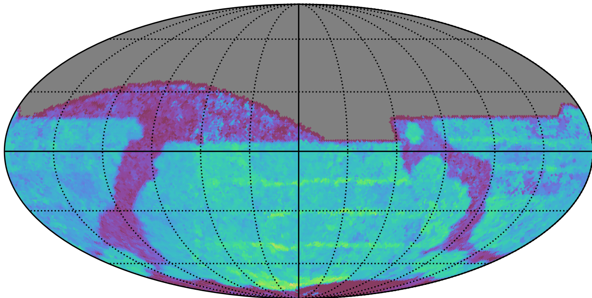
ddf_acor_sf25_lsf30_lsr10_v3.4_10yrs All sky z band: Median Season Length
