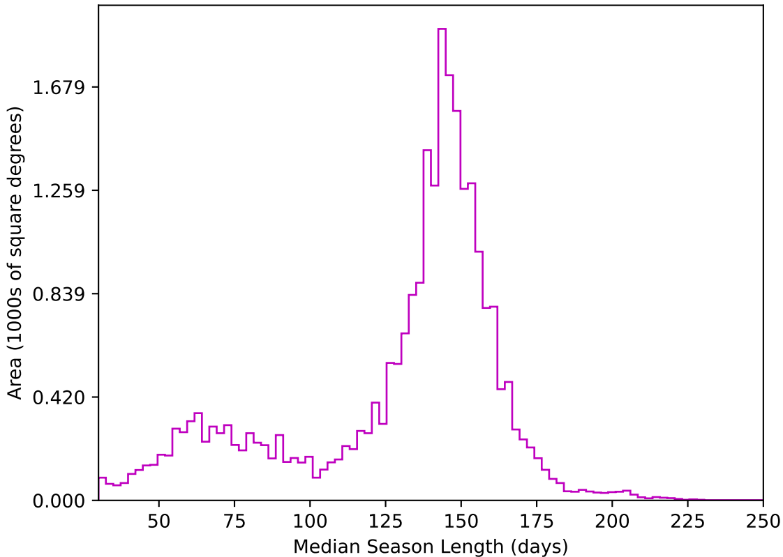
ddf_acor_sf25_lsf30_lsr10_v3.4_10yrs All sky z band: Median Season Length
