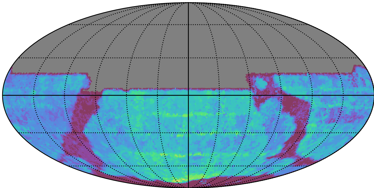
ddf_acor_sf25_lsf30_lsr10_v3.4_10yrs All sky y band: Median Season Length
