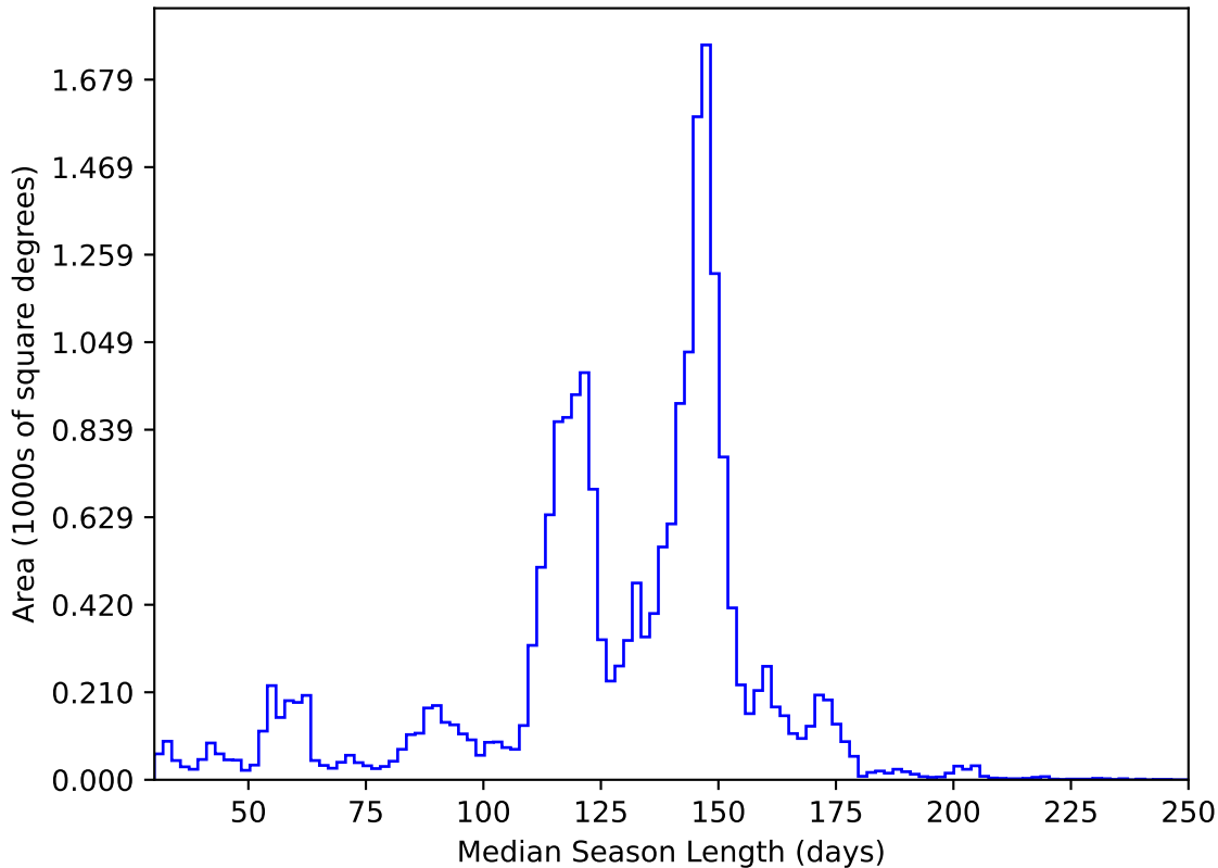
ddf_acor_sf25_lsf30_lsr10_v3.4_10yrs All sky y band: Median Season Length
