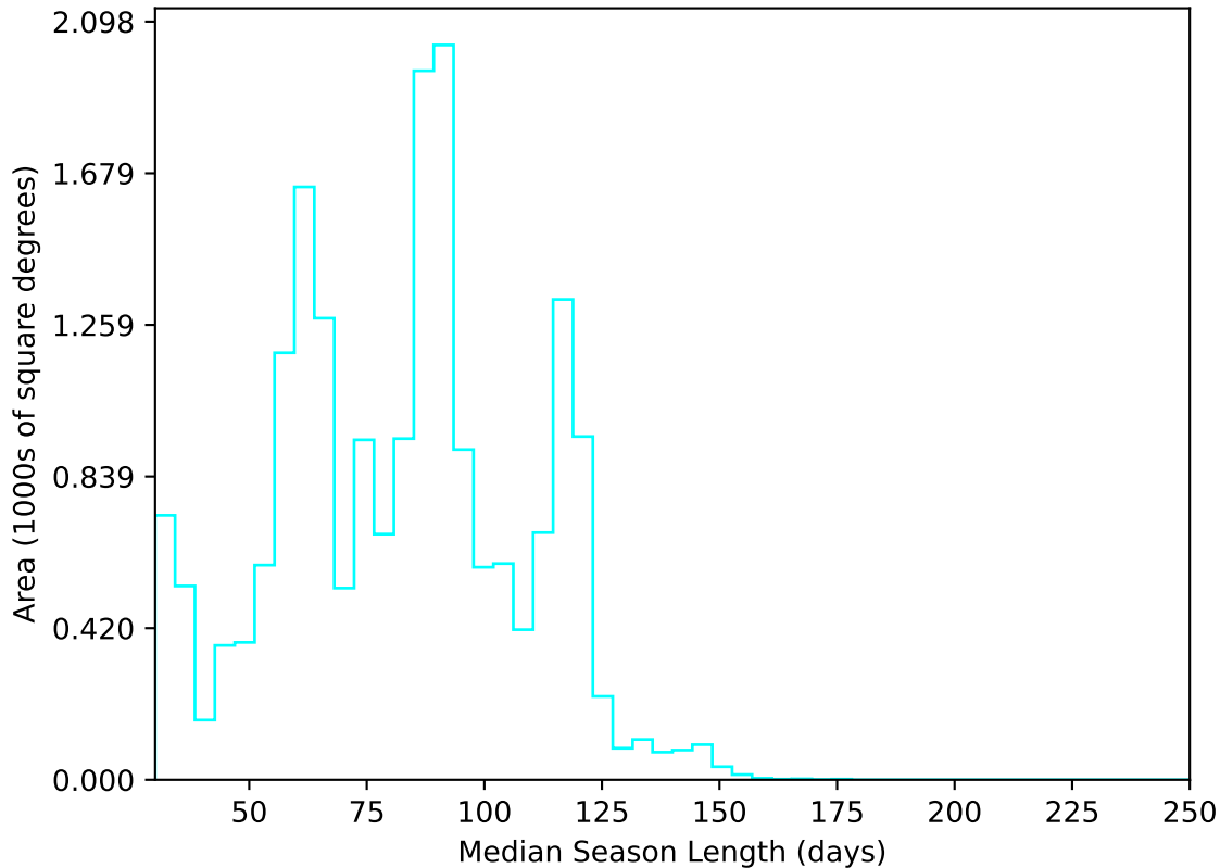
ddf_acor_sf25_lsf30_lsr10_v3.4_10yrs All sky u band: Median Season Length
