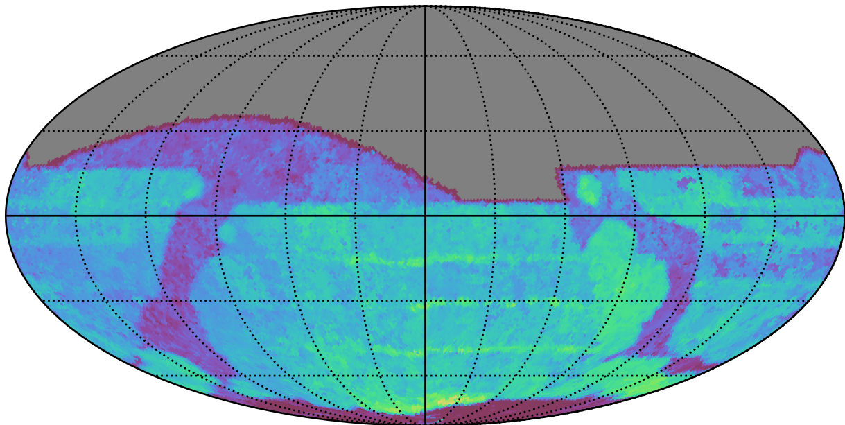
ddf_acor_sf25_lsf30_lsr10_v3.4_10yrs All sky r band: Median Season Length
