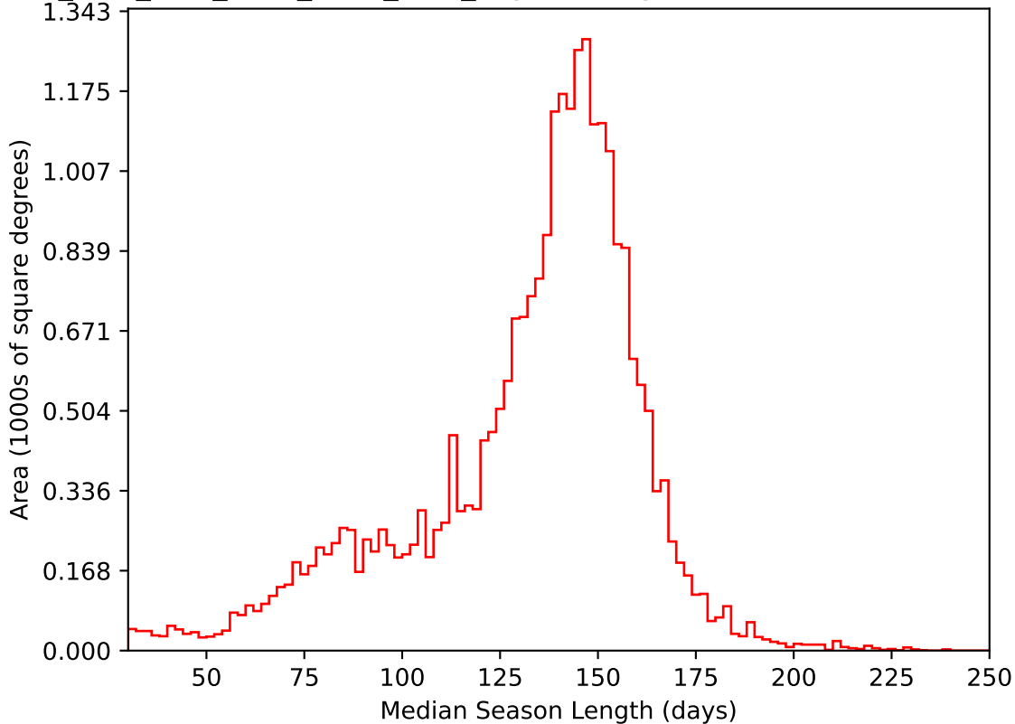
ddf_acor_sf25_lsf30_lsr10_v3.4_10yrs All sky i band: Median Season Length
