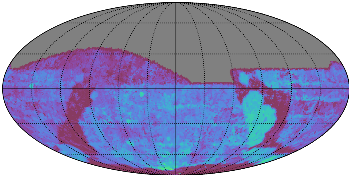
ddf_acor_sf25_lsf30_lsr10_v3.4_10yrs All sky g band: Median Season Length
