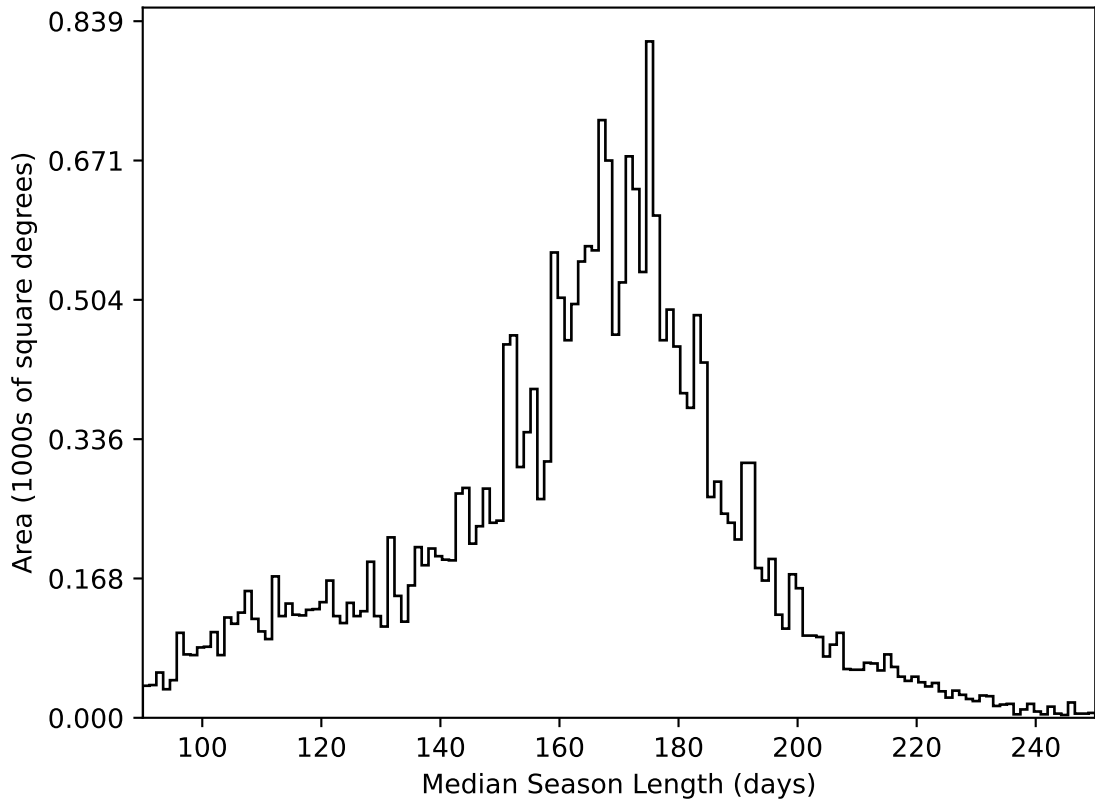
ddf_acor_sf25_lsf30_lsr10_v3.4_10yrs All sky all bands: Median Season Length
