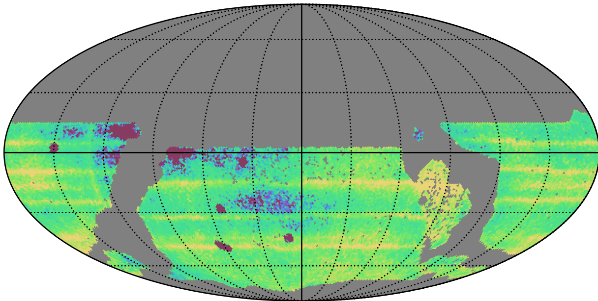
ddf_acor_sf25_lsf30_lsr10_v3.4_10yrs WFD: Median Intra-Night Gap
