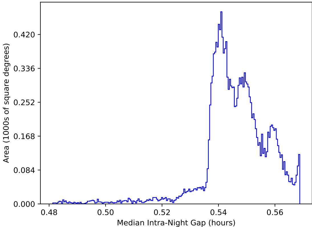
ddf_acor_sf25_ls30_lsr10_v3.4_10yrs WFD: Median Intra-Night Gap
