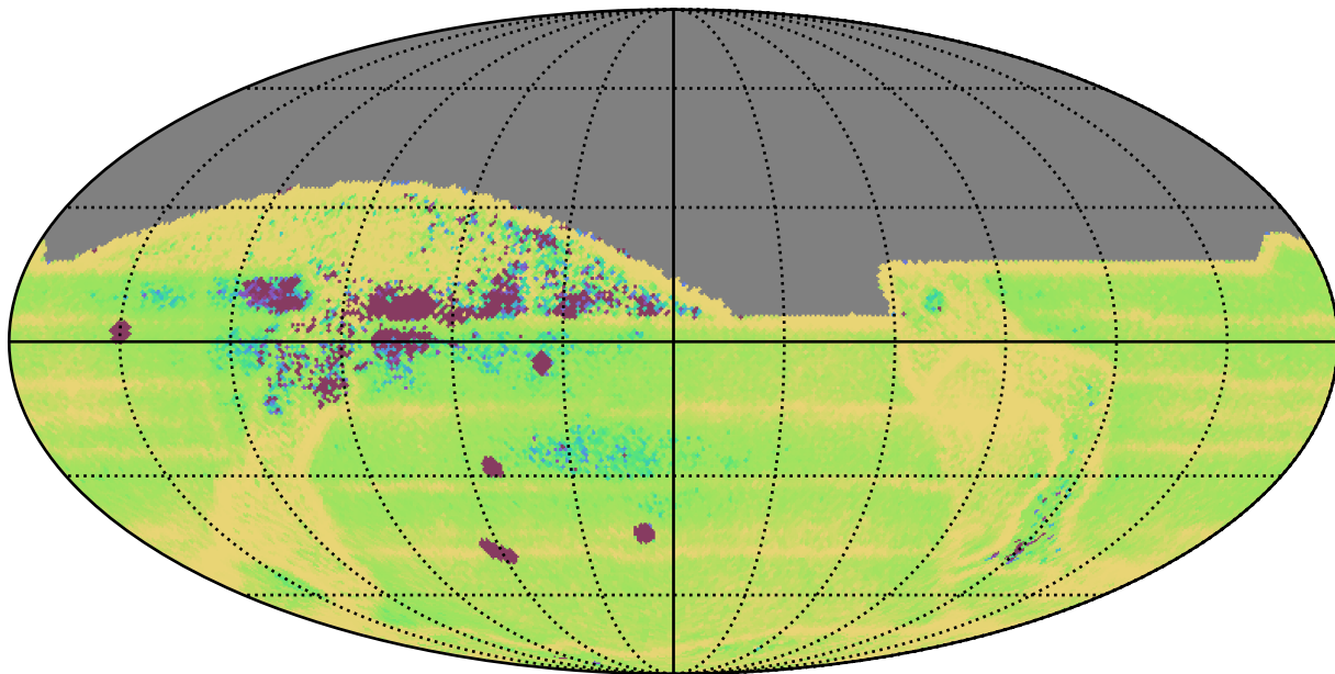
ddf_acor_sf25_lsf30_lsr10_v3.4_10yrs All sky: Median Intra-Night Gap
