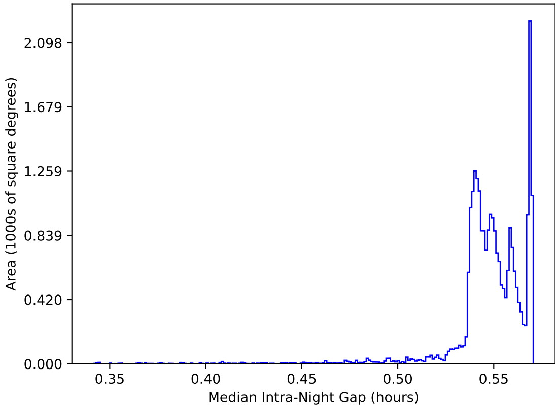
ddf_acor_sf25_lsf30_lsr10_v3.4_10yrs All sky: Median Intra-Night Gap
