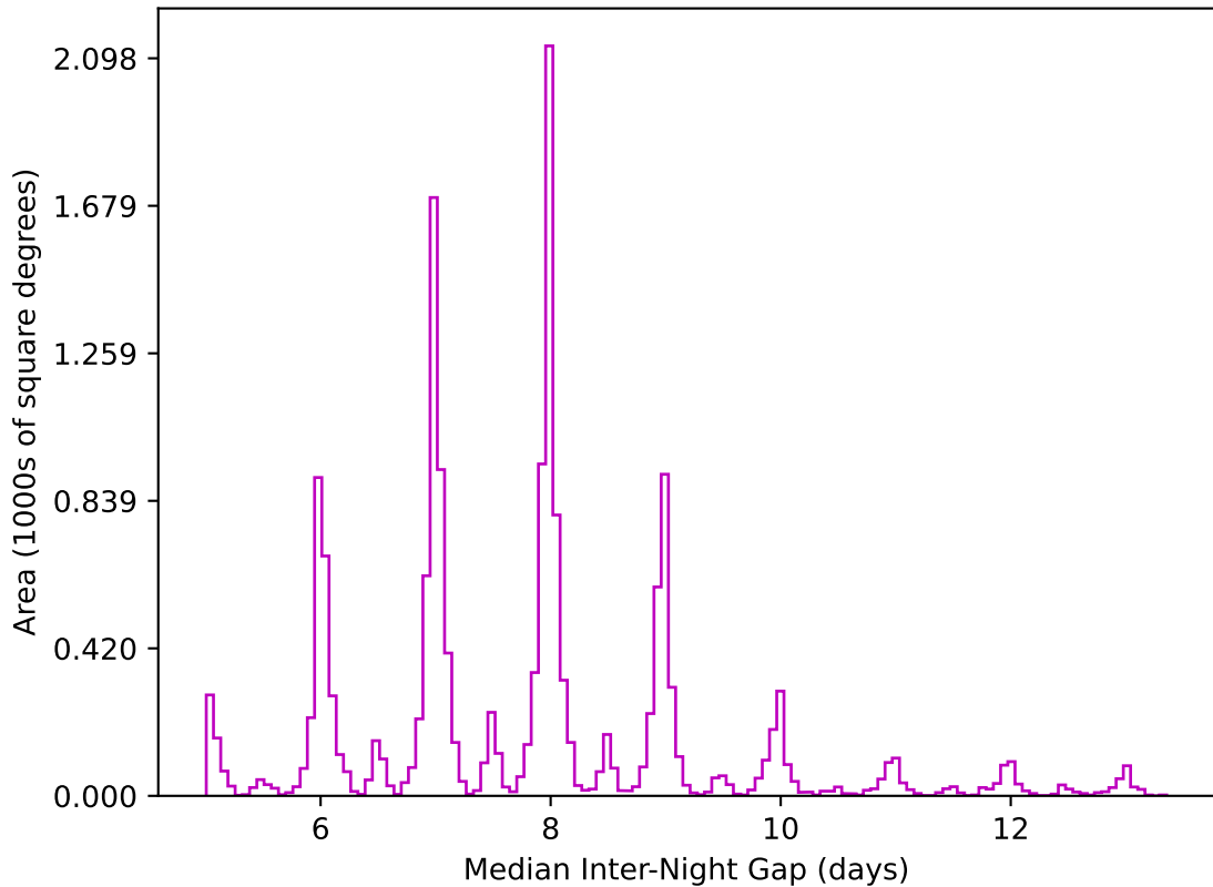
ddf_acor_sf25_lsf30_lsr10_v3.4_10yrs WFD z band: Median Inter-Night Gap
