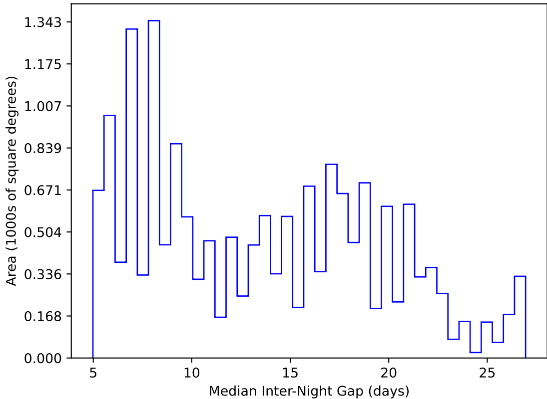
ddf_acor_sf25_lsf30_lsr10_v3.4_10yrs WFD y band: Median Inter-Night Gap
