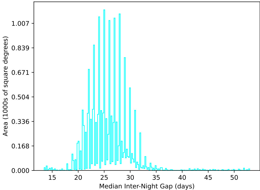
ddf_acor_sf25_lsf30_lsr10_v3.4_10yrs WFD u band: Median Inter-Night Gap
