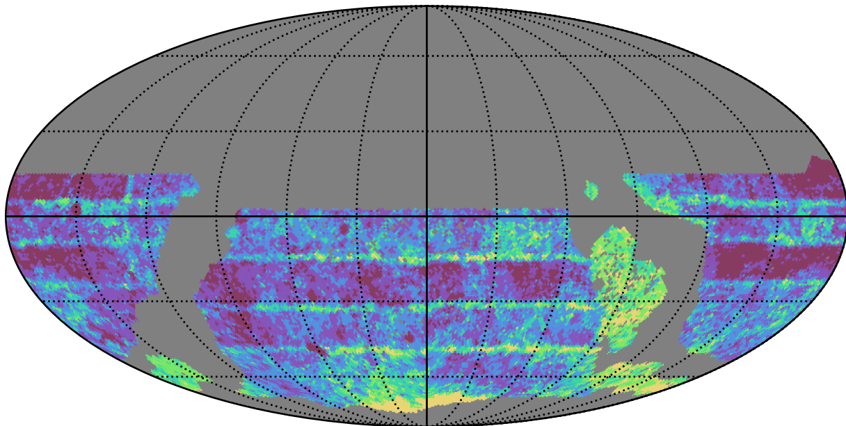
ddf_acor_sf25_lsf30_lsr10_v3.4_10yrs WFD r band: Median Inter-Night Gap
