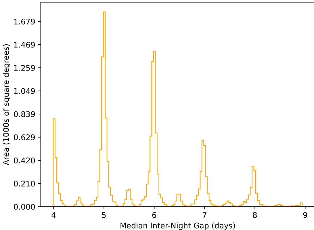
ddf_acor_sf25_lsf30_lsr10_v3.4_10yrs WFD r band: Median Inter-Night Gap
