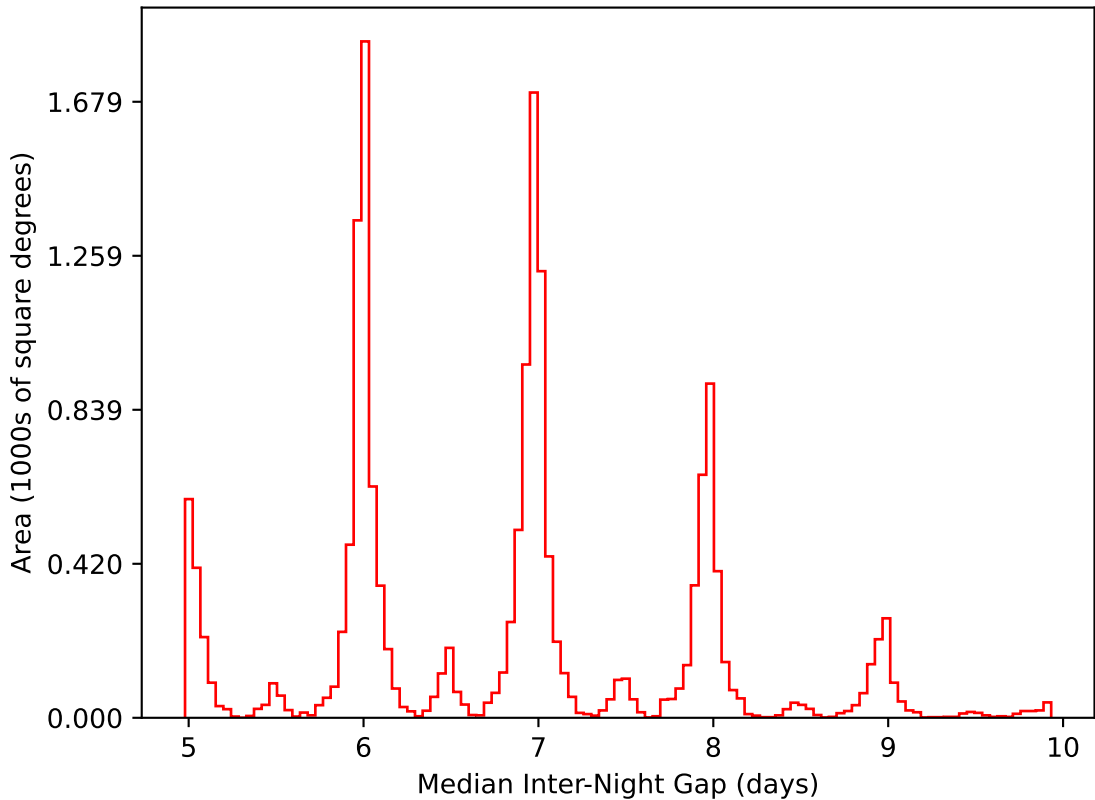
ddf_acor_sf25_lsf30_lsr10_v3.4_10yrs WFD i band: Median Inter-Night Gap
