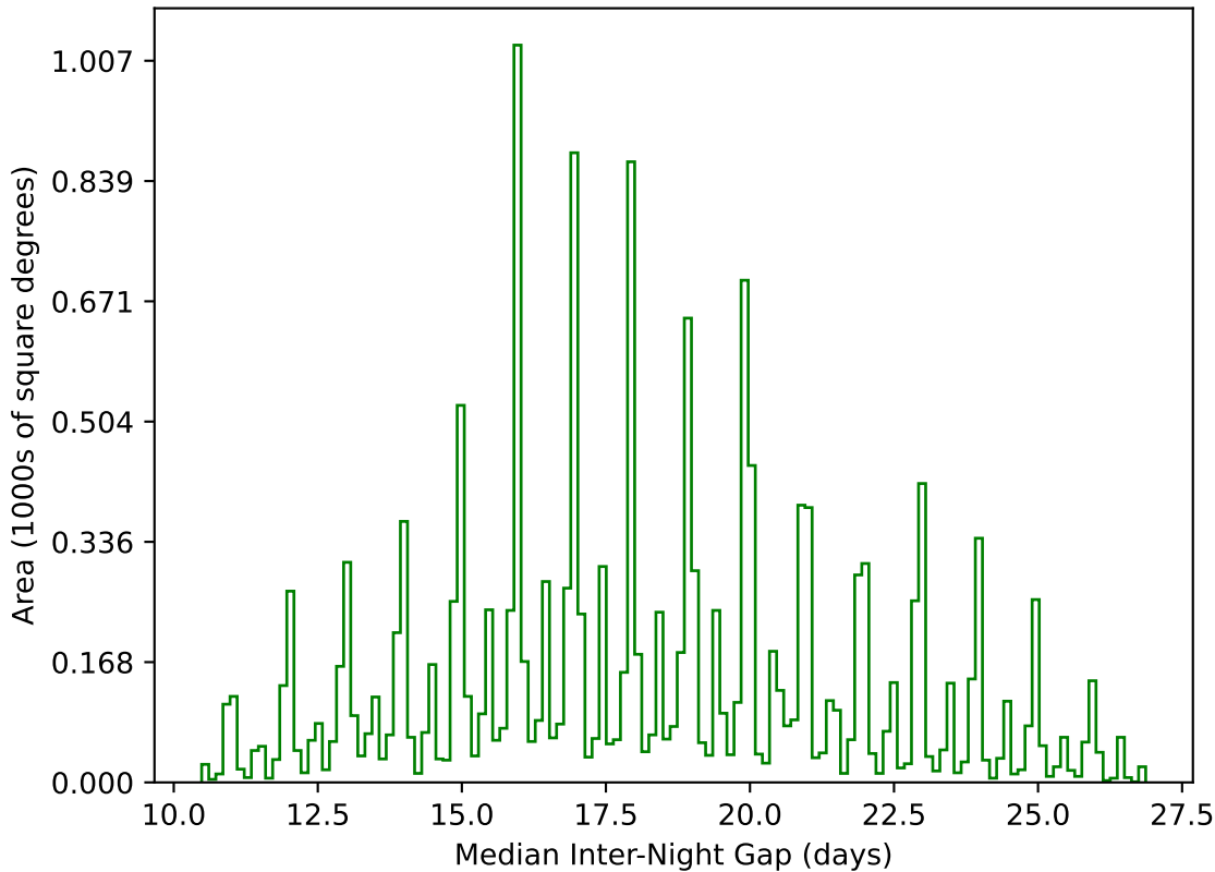
ddf_acor_sf25_lsf30_lsr10_v3.4_10yrs WFD g band: Median Inter-Night Gap
