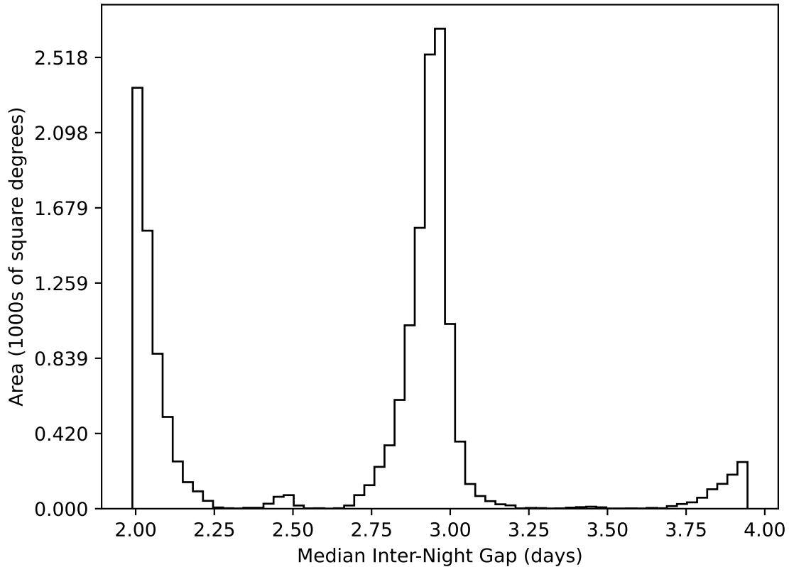
ddf_acor_sf25_lsf30_lsr10_v3.4_10yrs WFD all bands: Median Inter-Night Gap
