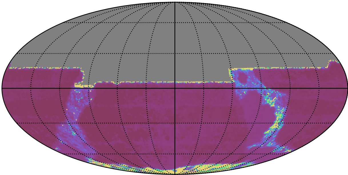
ddf_acor_sf25_lsf30_lsr10_v3.4_10yrs All sky y band: Median Inter-Night Gap
