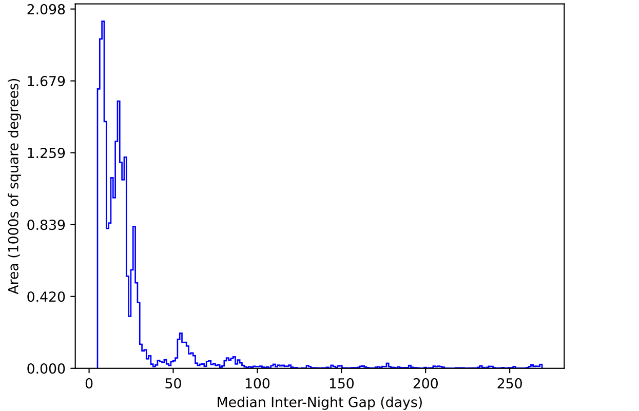
ddf_acor_sf25_lsf30_lsr10_v3.4_10yrs All sky y band: Median Inter-Night Gap
