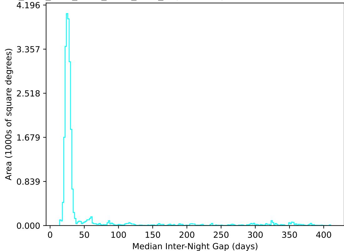
ddf_acor_sf25_lsf30_lsr10_v3.4_10yrs All sky u band: Median Inter-Night Gap
