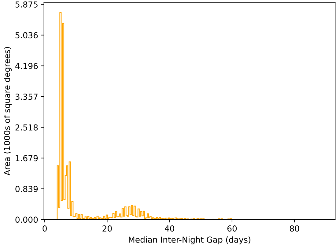
ddf_acor_sf25_lsf30_lsr10_v3.4_10yrs All sky r band: Median Inter-Night Gap
