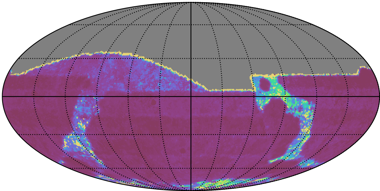
ddf_acor_sf25_lsf30_lsr10_v3.4_10yrs All sky g band: Median Inter-Night Gap
