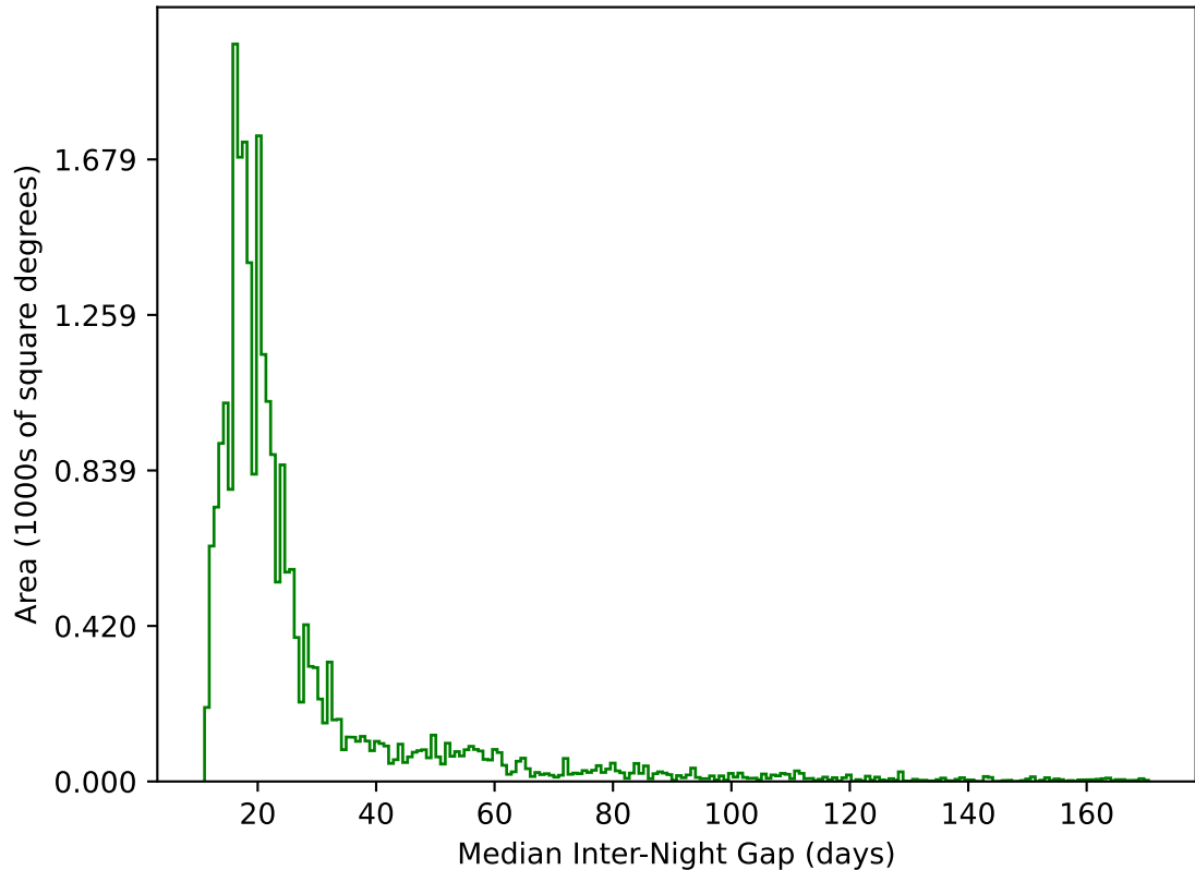
ddf_acor_sf25_lsf30_lsr10_v3.4_10yrs All sky g band: Median Inter-Night Gap
