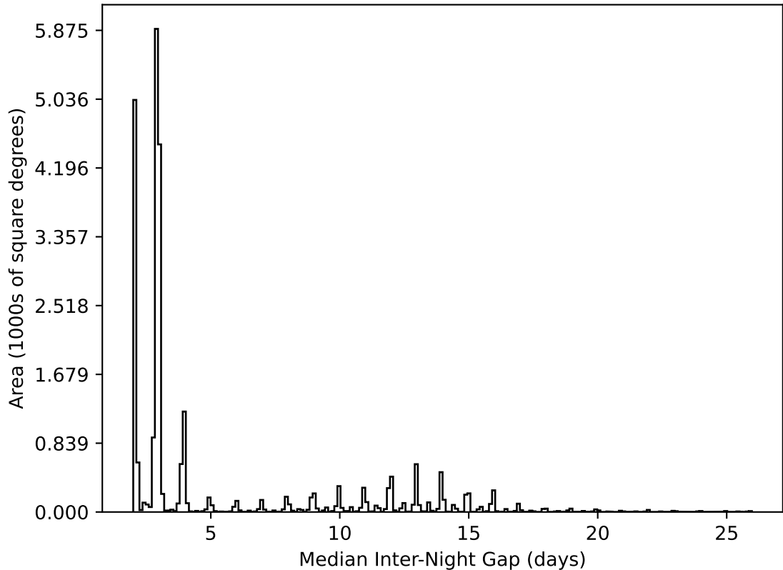
ddf_acor_sf25_lsf30_lsr10_v3.4_10yrs All sky all bands: Median Inter-Night Gap
