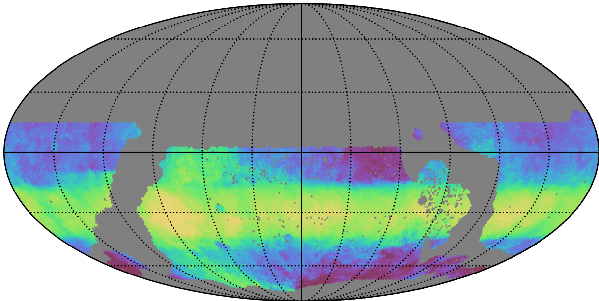
ddf_acor_sf25_lsf30_lsr10_v3.4_10yrs WFD z band: Median HA
