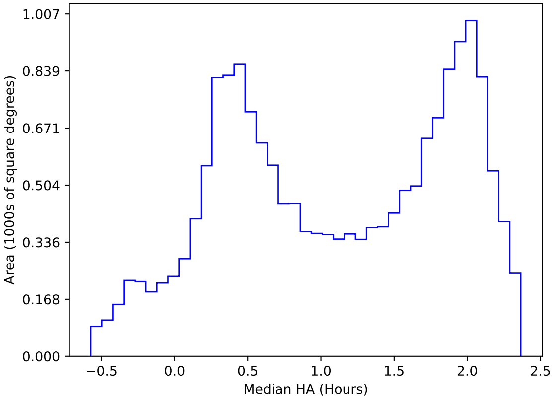
ddf_acor_sf25_lsf30_lsr10_v3.4_10yrs WFD z band: Median HA
