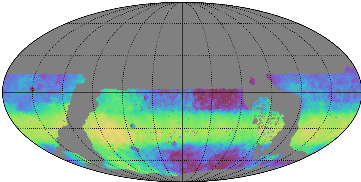
ddf_acor_sf25_lsf30_lsr10_v3.4_10yrs WFD y band: Median HA
