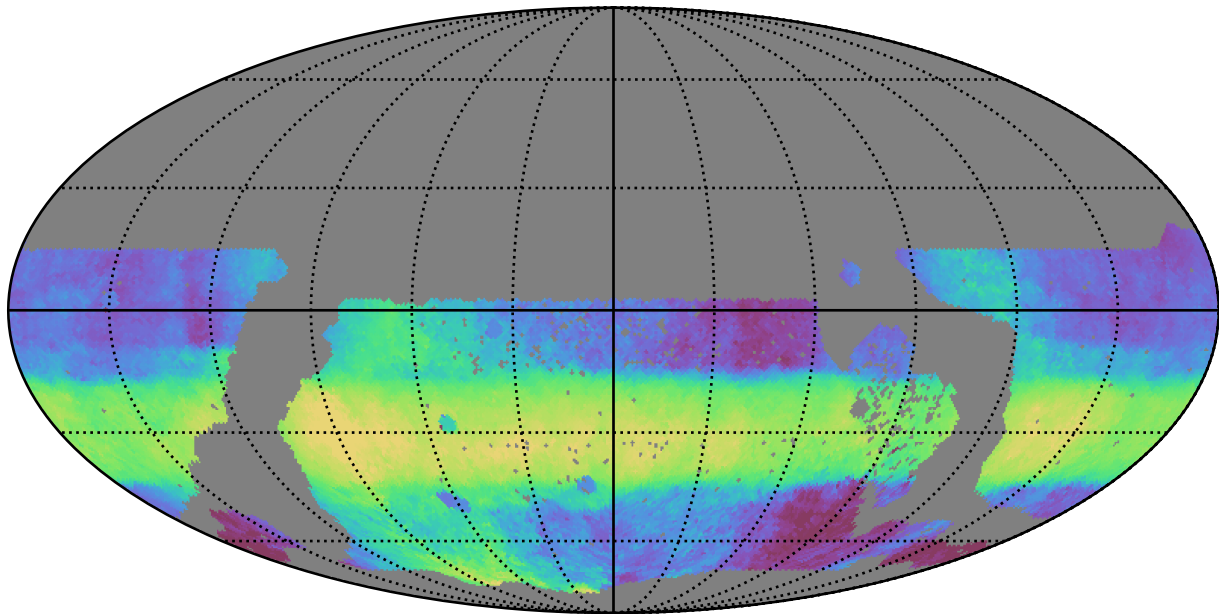
ddf_acor_sf25_lsf30_lsr10_v3.4_10yrs WFD r band: Median HA
