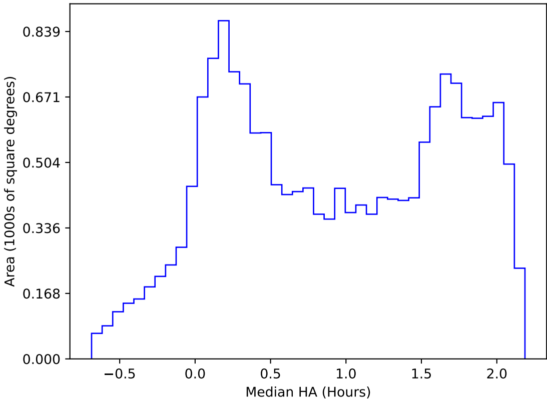
ddf_acor_sf25_lsf30_lsr10_v3.4_10yrs WFD r band: Median HA
