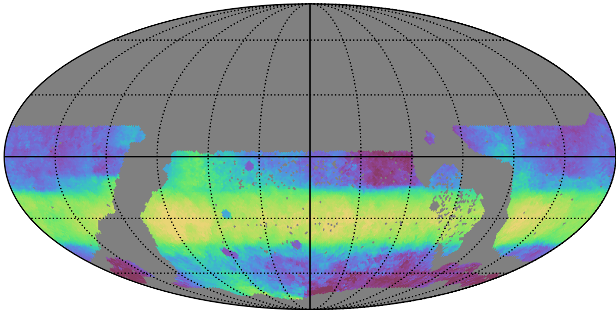
ddf_acor_sf25_lsf30_lsr10_v3.4_10yrs WFD i band: Median HA
