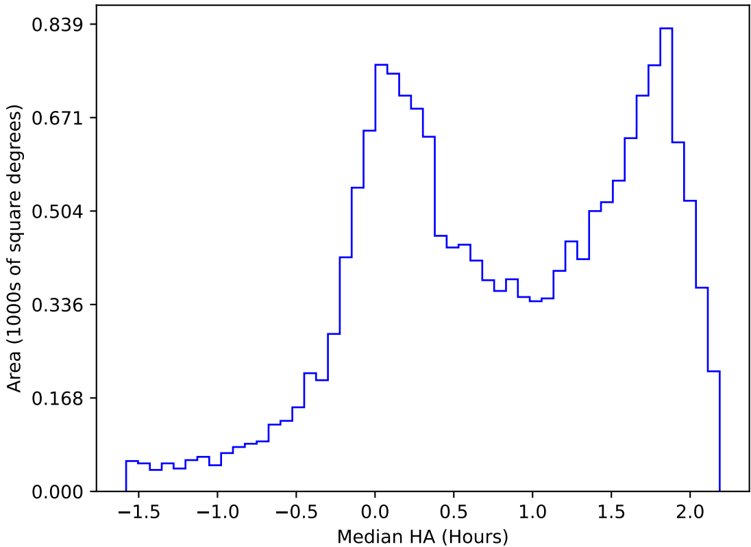
ddf_acor_sf25_lsf30_lsr10_v3.4_10yrs WFD g band: Median HA
