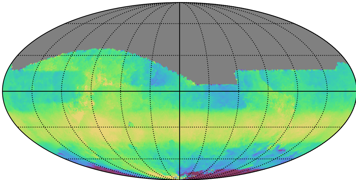
ddf_acor_sf25_lsf30_lsr10_v3.4_10yrs All sky z band: Median HA
