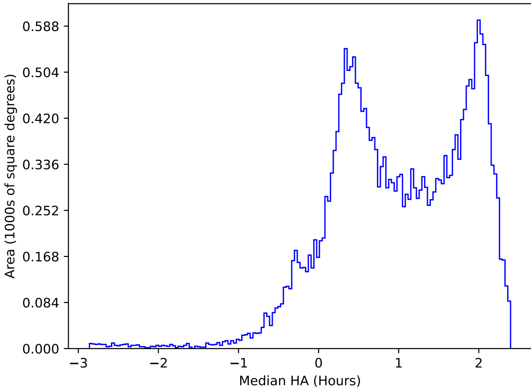
ddf_acor_sf25_lsf30_lsr10_v3.4_10yrs All sky z band: Median HA
