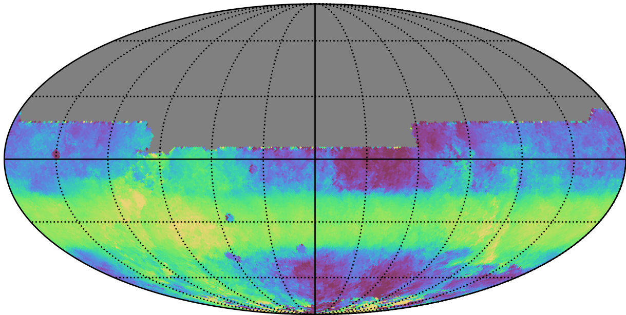
ddf_acor_sf25_lsf30_lsr10_v3.4_10yrs All sky y band: Median HA
