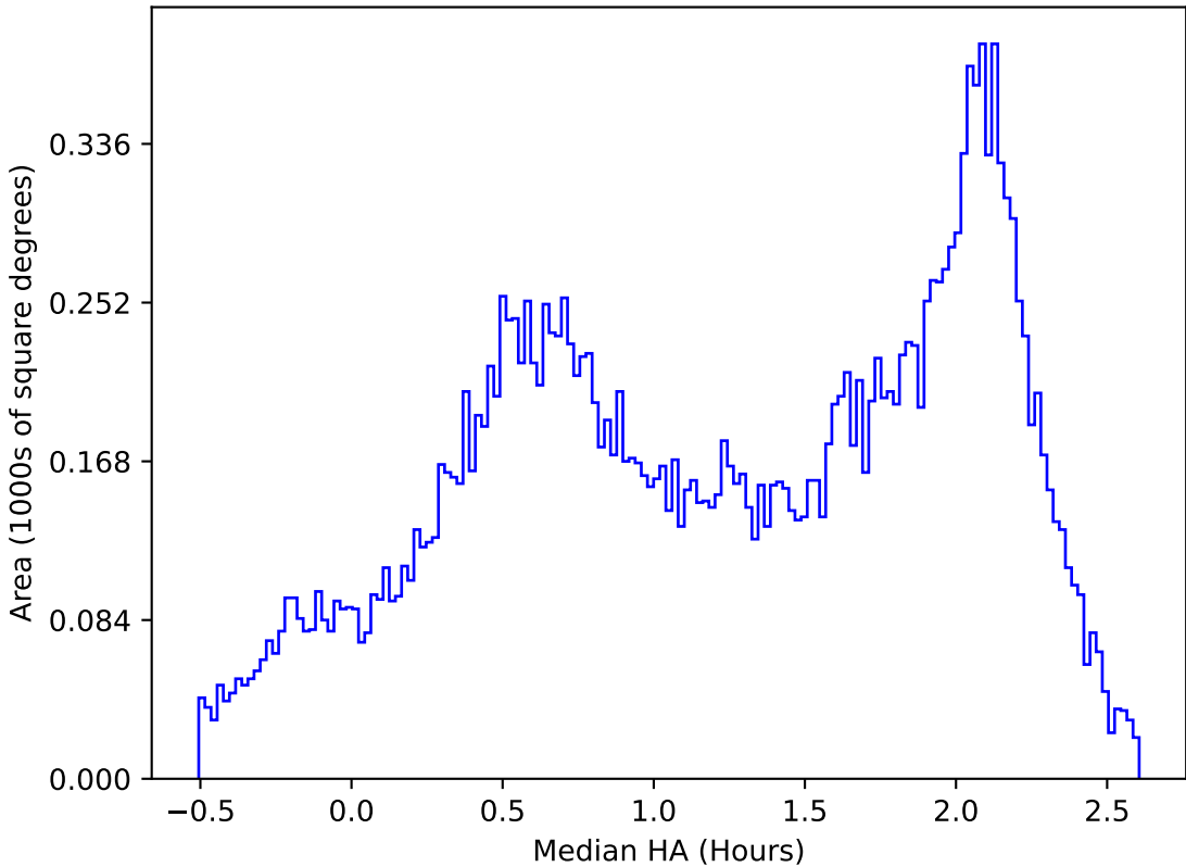
ddf_acor_sf25_ls30_lsr10_v3.4_10yrs All sky y band: Median HA
