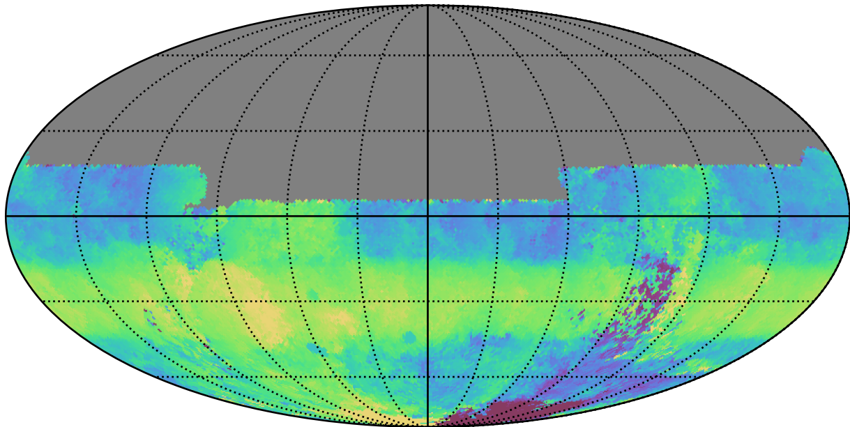
ddf_acor_sf25_lsf30_lsr10_v3.4_10yrs All sky u band: Median HA
