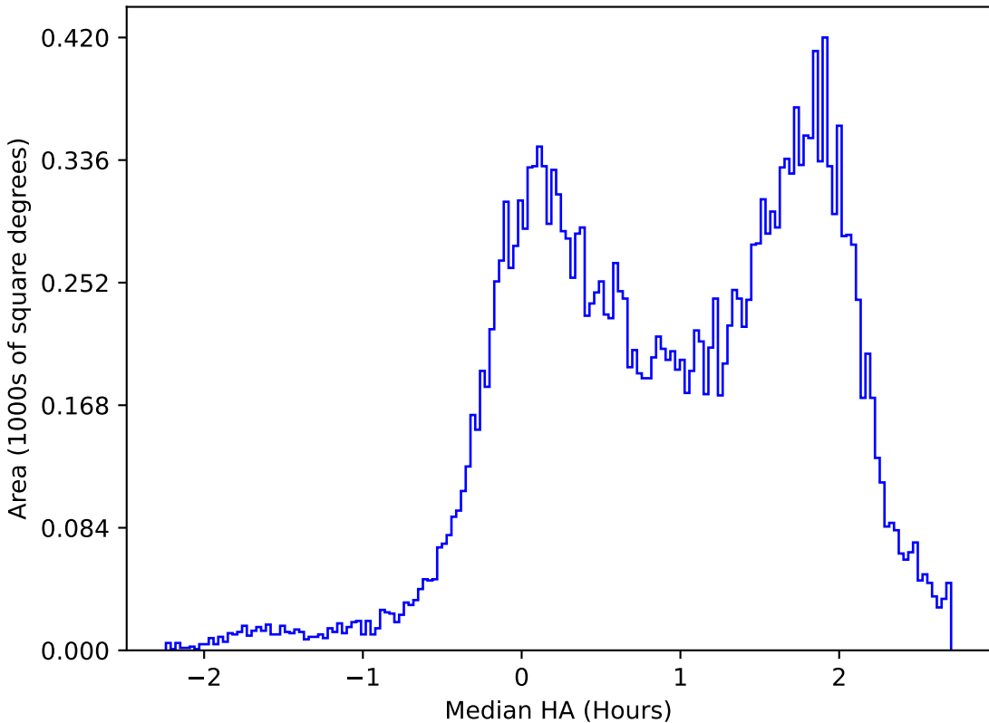
ddf_acor_sf25_ls30_lsr10_v3.4_10yrs All sky u band: Median HA
