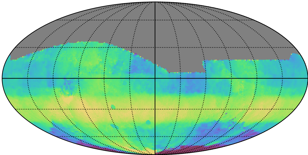
ddf_acor_sf25_lsf30_lsr10_v3.4_10yrs All sky r band: Median HA
