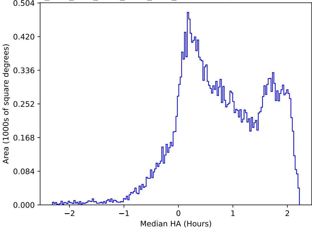
ddf_acor_sf25_lsf30_lsr10_v3.4_10yrs All sky r band: Median HA
