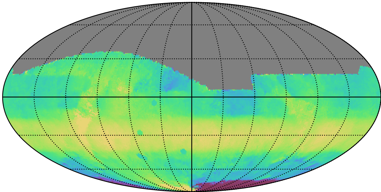
ddf_acor_sf25_lsf30_lsr10_v3.4_10yrs All sky i band: Median HA
