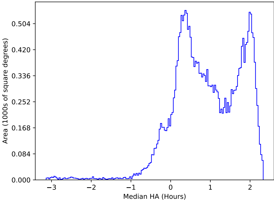
ddf_acor_sf25_lsf30_lsr10_v3.4_10yrs All sky i band: Median HA
