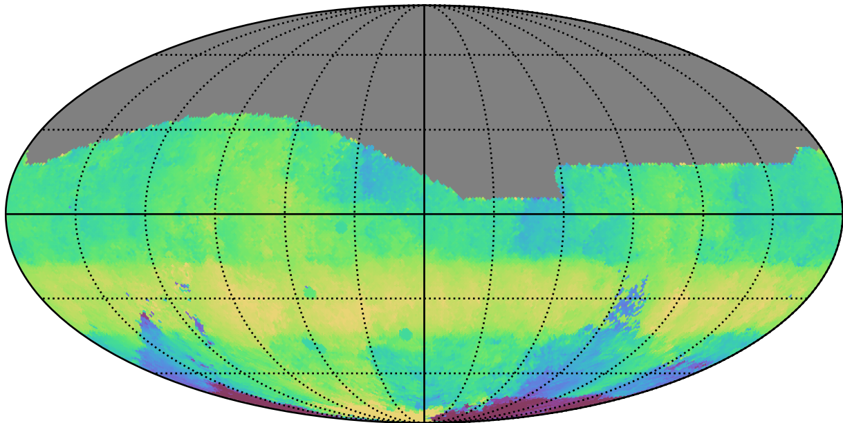
ddf_acor_sf25_lsf30_lsr10_v3.4_10yrs All sky g band: Median HA
