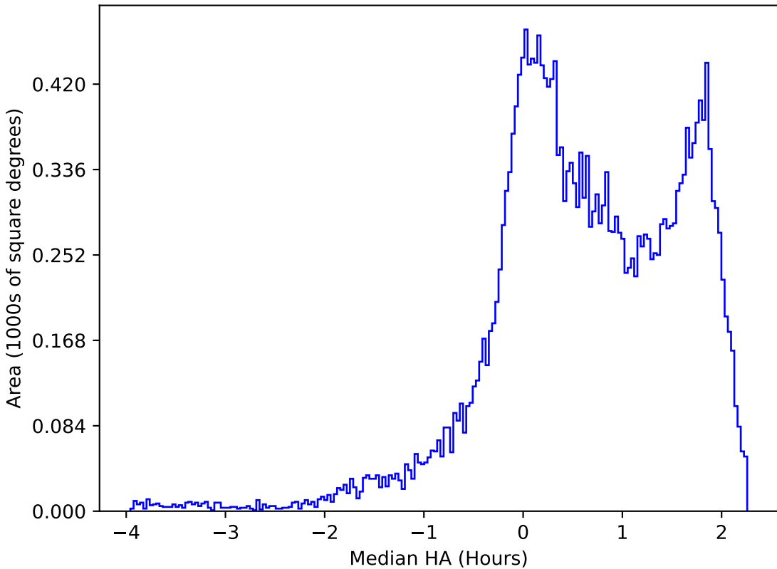
ddf_acor_sf25_lsf30_lsr10_v3.4_10yrs All sky g band: Median HA
