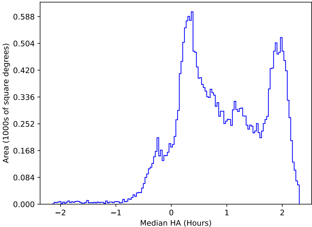
ddf_acor_sf25_lsf30_lsr10_v3.4_10yrs All sky all bands: Median HA
