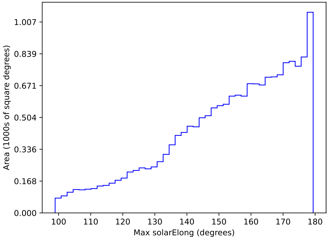
ddf_acor_sf25_lsf30_lsr10_v3.4_10yrs WFD z band: Max solarElong
